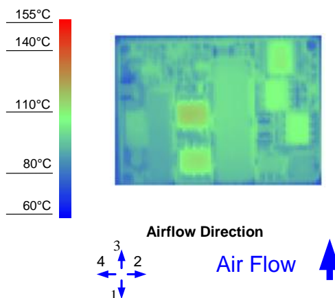
Figure 8. Thermal Image for Airflow Direction 3 (10A output, 55°C ambient, 0 LFM, typical Vin, open frame, unit soldered onto a fixture board)
